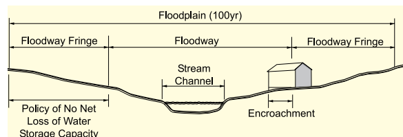
Floodplain Diagram
