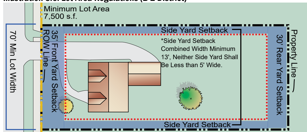
Illustration 3.6: Lot Area Regulations (B-2 District)
