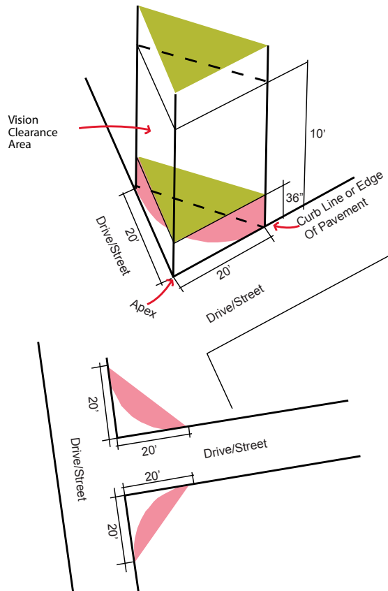
Illustration 5.15: Site Vision Triangle
