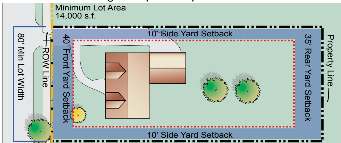
Illustration 3.4: Lot Area Regulations (A-2 District)
