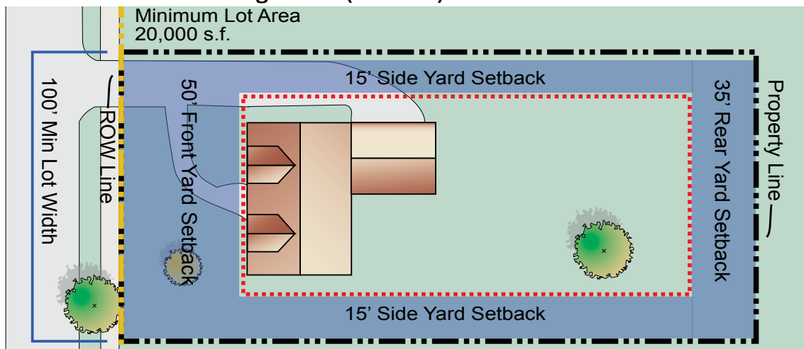
Illustration 3.3: Lot Area Regulations (A District)
