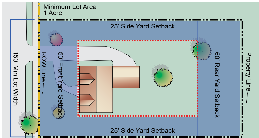
Illustration 3.1: Lot Area Regulations (A-A District)
