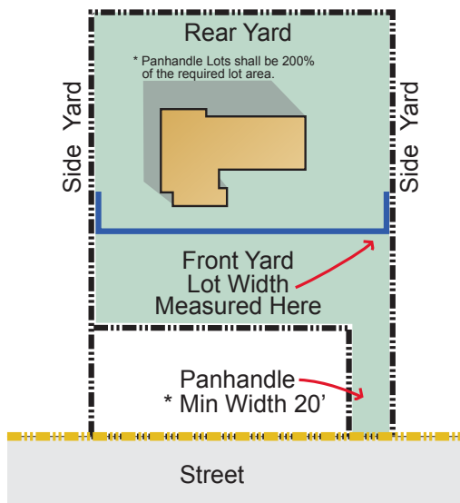
Illustration 5.2: Lot Panhandle Diagram
