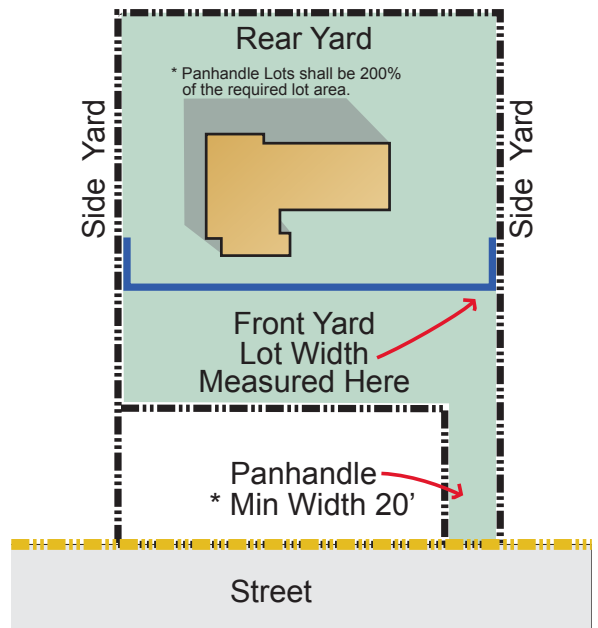
Lot Panhandle Diagram
