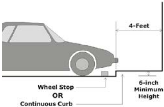
Illustration 5.7: Placement
